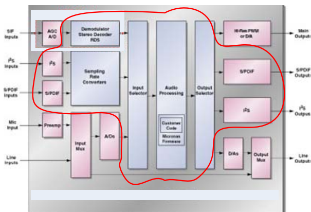
Multi channel audio IC architecture (FPGA design architecture circled)
